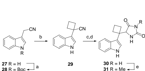
Scheme 5. Reagents and conditions: (a) \text{Boc}_2\text{O} , DMAP, \text{CH}_2\text{Cl}_2 , rt (76%); (b) \text{NaH} , \text{Br}(\text{CH}_2)_3\text{Br} , \text{DMSO} , 0^\circ\text{C} to rt, 16 h (75%); (c) DIBAL, toluene, -50^\circ\text{C} then \text{Et}_2\text{O}-\text{NH}_4\text{Cl} (1:1) then 2 N \text{H}_2\text{SO}_4 (68%); (d) (\text{NH}_4)_2\text{CO}_3 , \text{KCN} , \text{EtOH} , \text{H}_2\text{O} , 80^\circ\text{C} (63%); (e) DMA–DMA, toluene/DMF (5:1), 110^\circ\text{C} , 2 h (98%).
