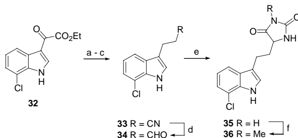
Scheme 6. Reagents and conditions: (a) \text{LiAlH}_4 , \text{THF} , \Delta , 18 h (75%); (b) \text{PPh}_3 , imidazole, \text{I}_2 , \text{DCM} , rt, 1.5 h (85%); (c) \text{KCN} , \text{DMF} , 110^\circ\text{C} 4 h (95%); (d) DIBAL, toluene, -70^\circ\text{C} to rt, 5 h (51%); (e) (\text{NH}_4)_2\text{CO}_3 , \text{KCN} , \text{EtOH} , \text{H}_2\text{O} , 60^\circ\text{C} , 20 h (78%); (f) DMA–DMA, toluene, \Delta , 2 h (65%).
