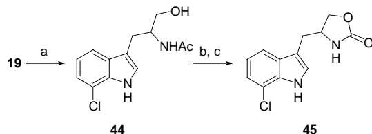
Scheme 8. Reagents and conditions: (a) \text{BH}_3\cdot\text{THF} , -5^\circ\text{C} to rt, 4 h (74%); (b) 3 N HCl, \Delta , 4 h; (c) CDI, \text{Et}_3\text{N} , -5^\circ\text{C} to rt, 24 h (42% over two steps).
