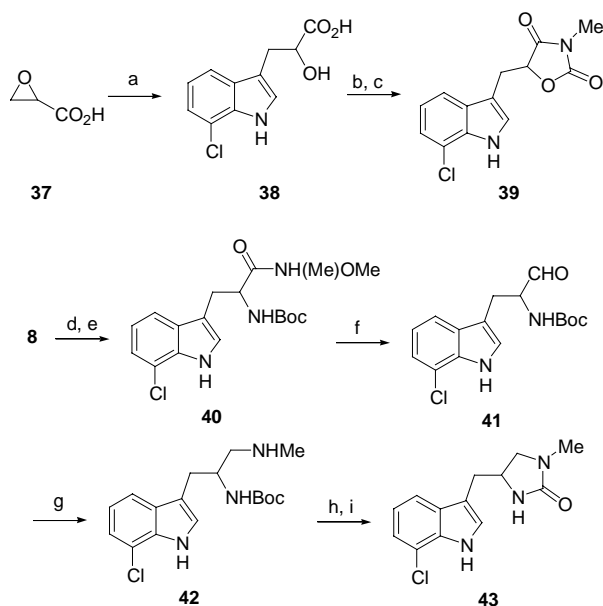
Scheme 7. Reagents and conditions: (a) 4 , \text{SnCl}_4 , \text{CCl}_4 , 0^\circ\text{C} , 1.5 h (7%); (b) HBTU, \text{MeNH}_2 in THF, \text{CH}_2\text{Cl}_2 , i\text{-Pr}_2\text{EtN} , rt, 12 h (25%); (c) CDI, THF, rt, 36 h (38%); (d) \text{Boc}_2\text{O} , satd aq \text{NaHCO}_3 , \text{EtOAc} /THF (10:3), rt, 12 h (80%); (e) HBTU, \text{NH}(\text{Me})\text{OMeHCl} , \text{CH}_2\text{Cl}_2 , i\text{-Pr}_2\text{EtN} , rt, 1 h (78%); (f) \text{LiAlH}_4 , THF, -50^\circ\text{C} , 1 h; (g) \text{MeNH}_2 in THF, \text{MgSO}_4 , rt, 3 h then \text{NaBH}_4 (10 equiv), 0^\circ\text{C} , 2 h (40% for two steps); (h) satd HCl in MeOH, rt, 2 h; (i) CDI, \text{Et}_3\text{N} , 0^\circ\text{C} to rt, 24 h (45% for two steps).
